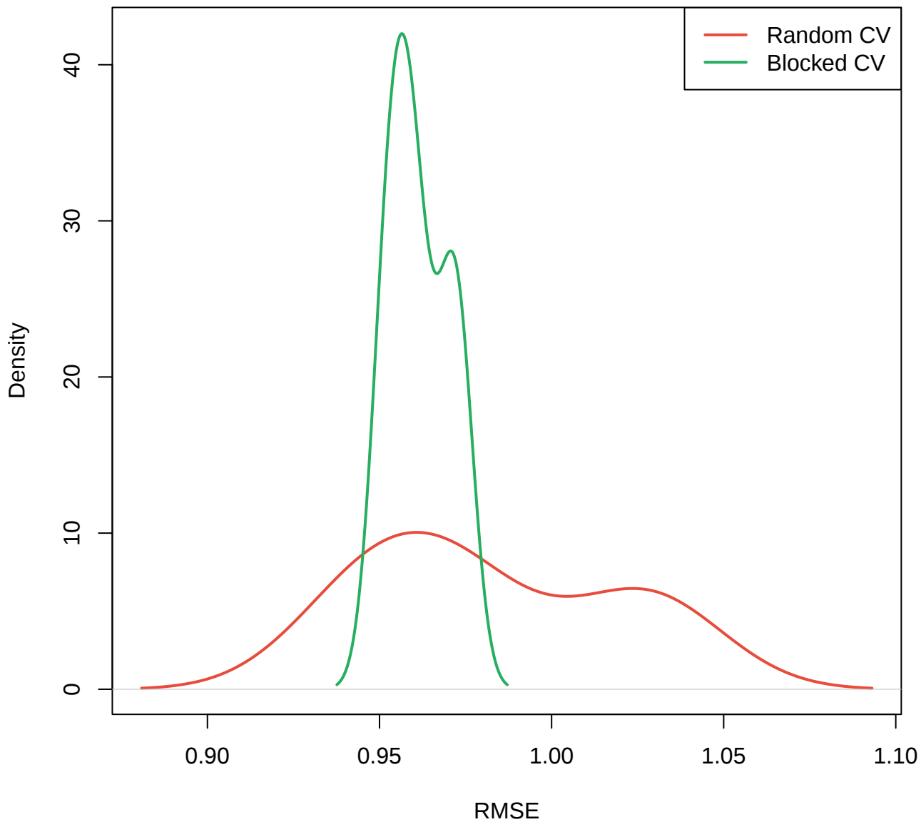
Distribution of CV Estimates
