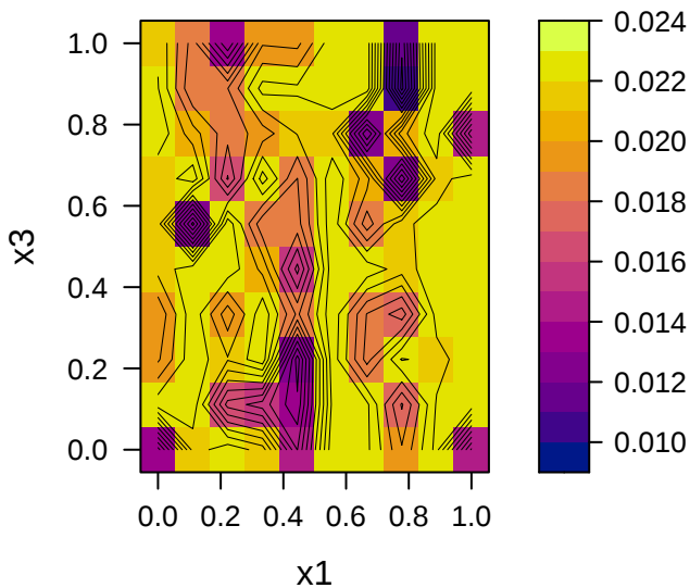
Predictive Variance
