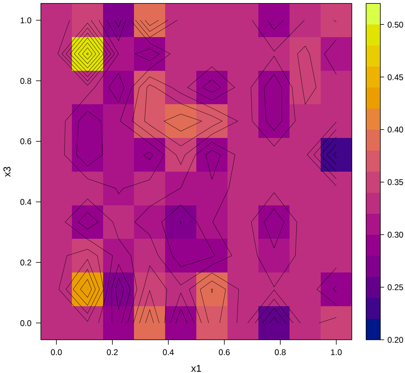
Predictive Mean
