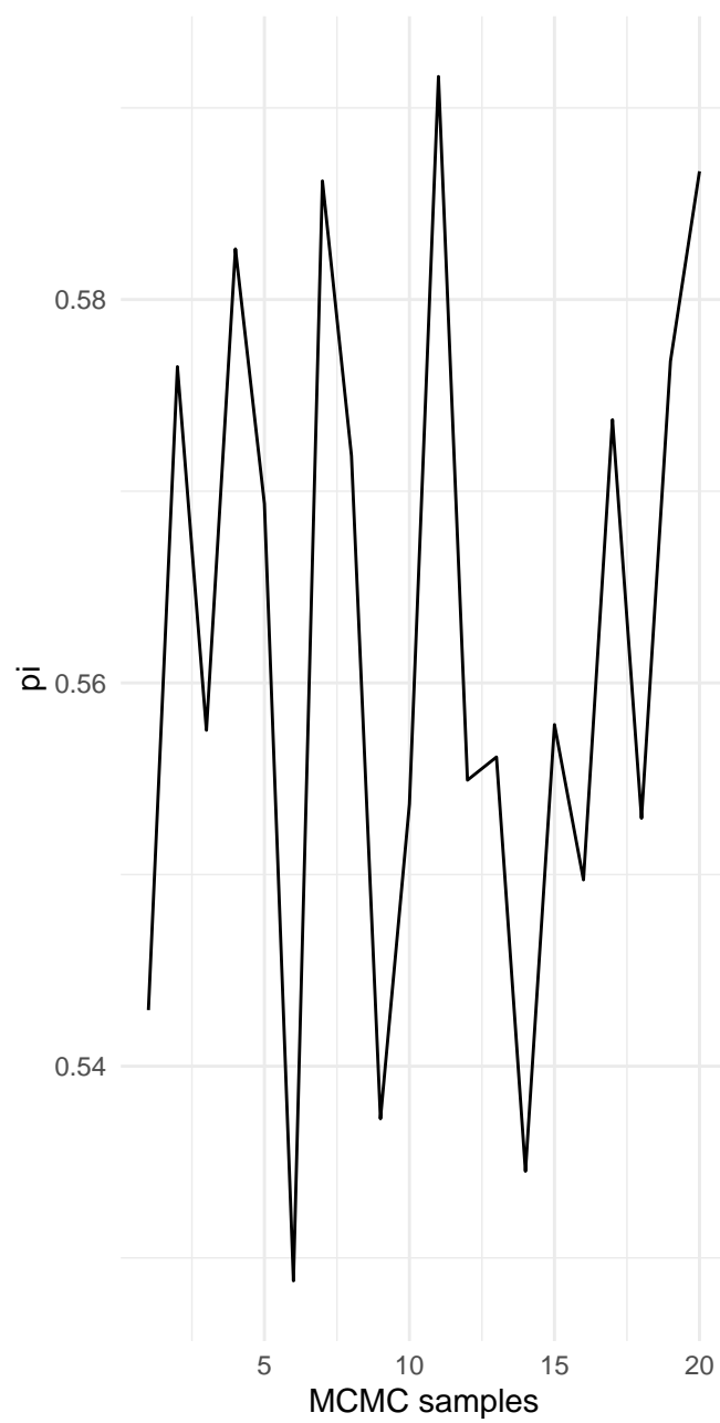
Cluster 2
