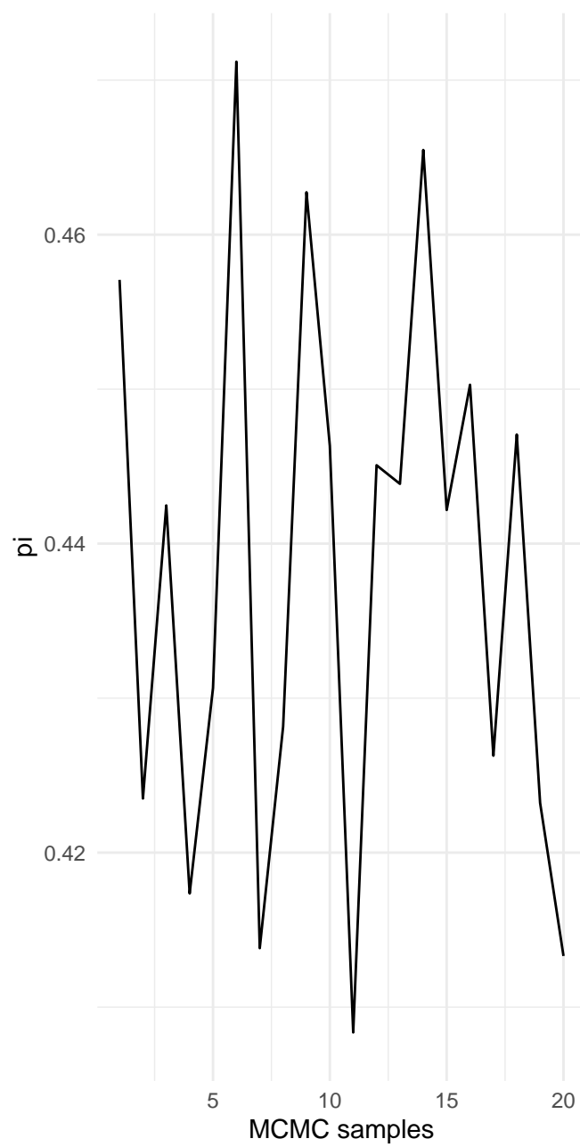
Cluster 1
