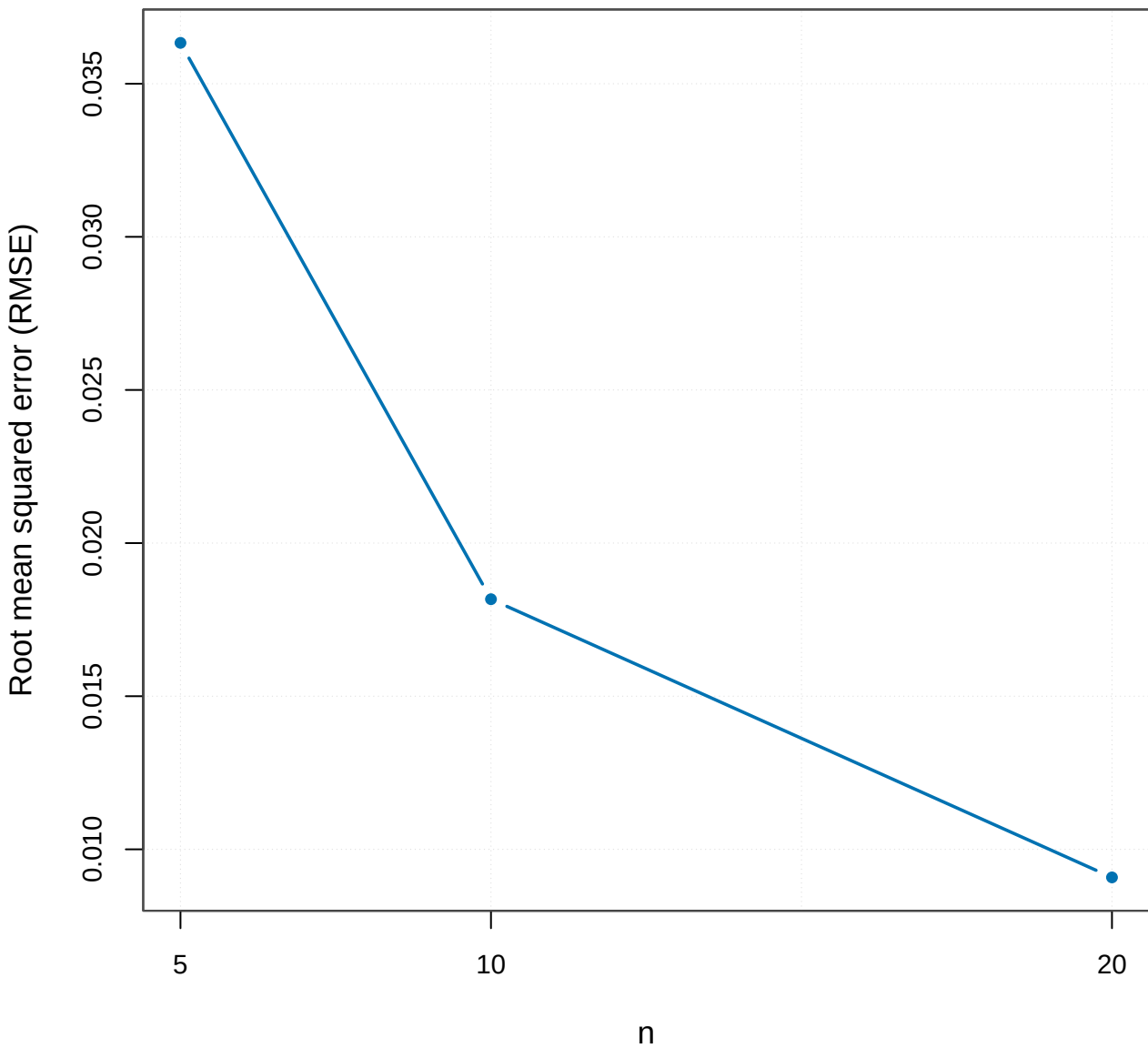
Root mean squared error versus n
