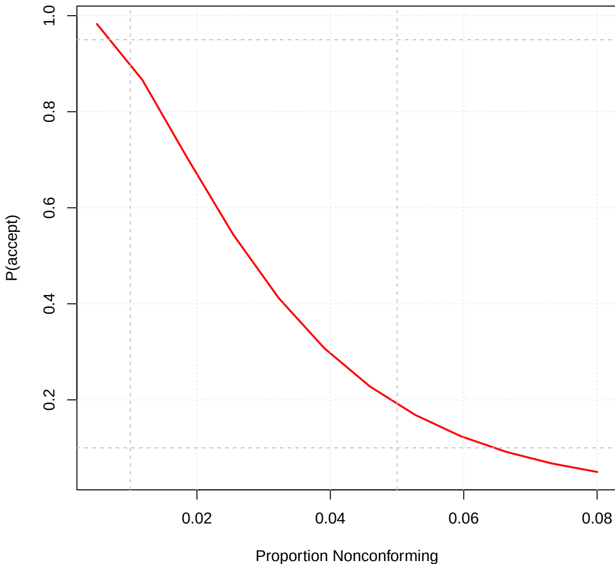
Variables Sampling OC Curve by Pd | n=45, k=2.2 | beta
