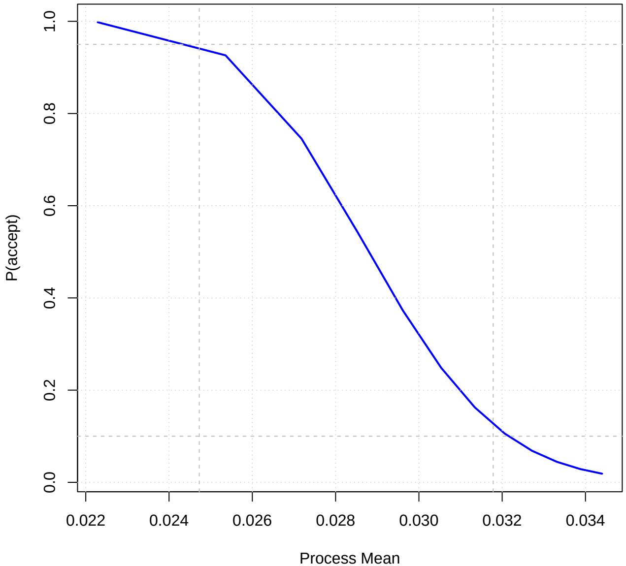
Variables Sampling OC Curve by Mean | n=45, k=2.2 | beta
