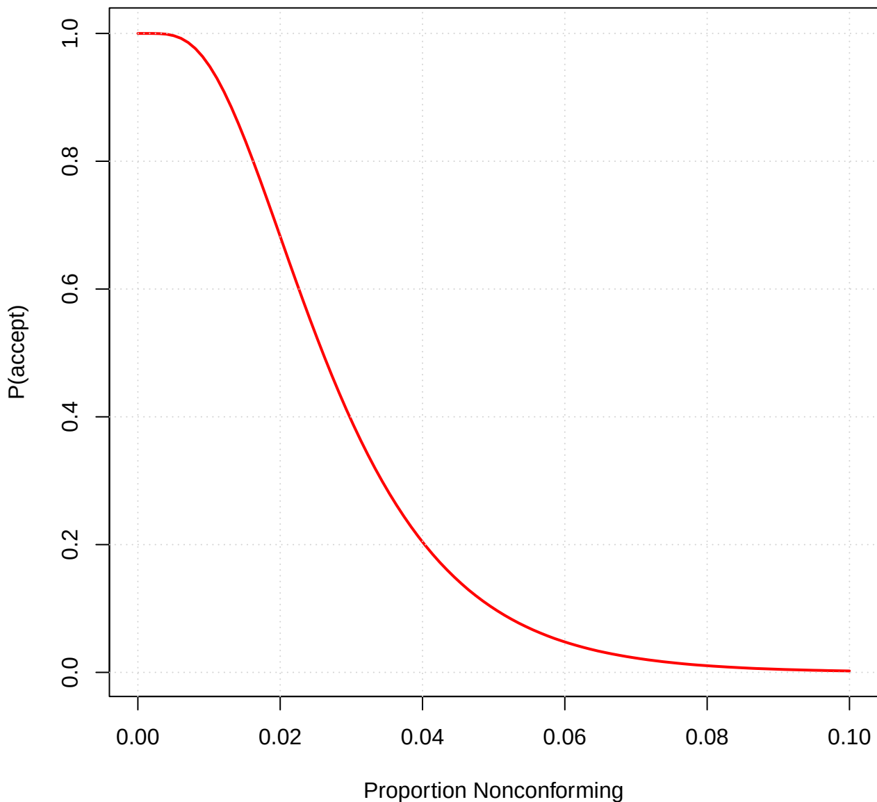
OC Curve by Proportion Nonconforming
