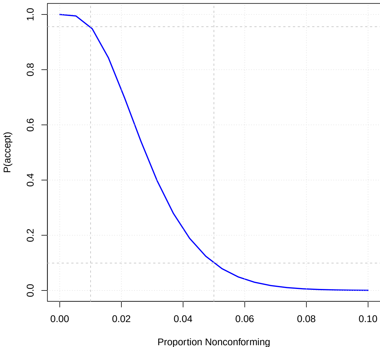
Attributes Sampling OC Curve | n=132, c=3 | binomial
