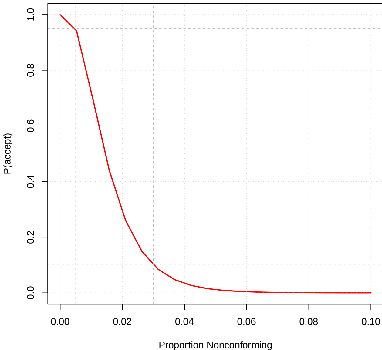
Variables Sampling OC Curve by Pd | n=18, k=2.185 | normal
